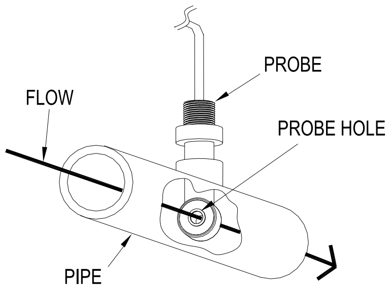
Fig. 1: Typical Installation
