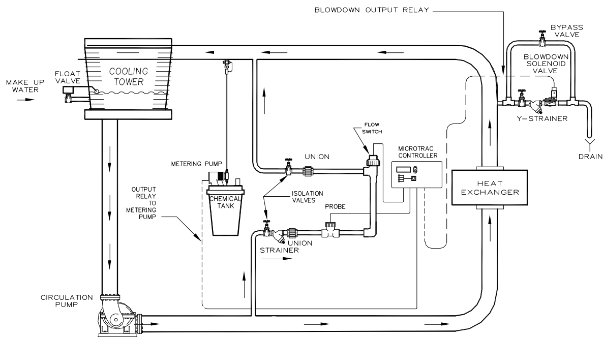
Fig. 1: Typical Installation
